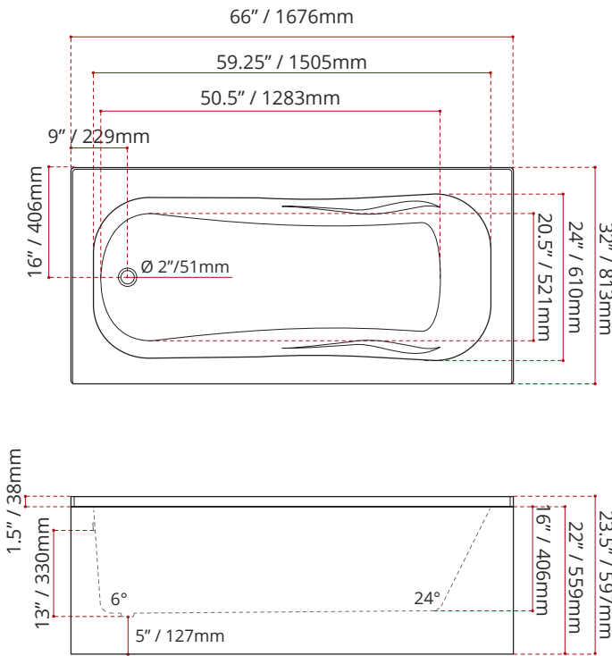
MODEL NUMBER : 4351 (LEFT HAND DRAIN LOCATION)
