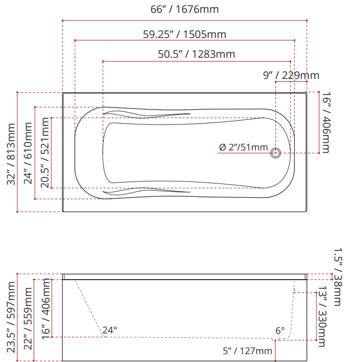
MODEL NUMBER : 4361 (RIGHT HAND DRAIN LOCATION)
